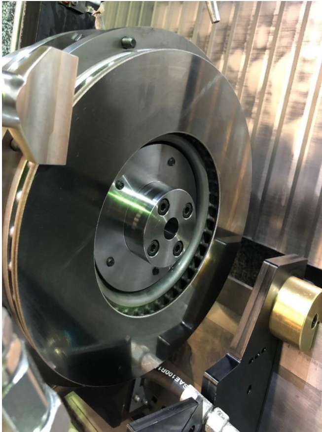
Image 2: A finished brake disc coated with the EHLA process.
